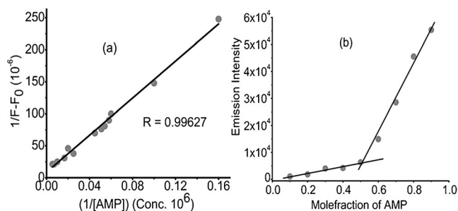
Figure 5. Determination of K_a for the interaction of [\text{Eu}_2(\text{H}_2\text{L})_2(\text{NO}_3)_2(\text{H}_2\text{O})_4](\text{NO}_3)_4 with AMP by the Benesi–Hildebrand method (a) and the corresponding Job plot (b), confirming the 1:1 stoichiometry.
