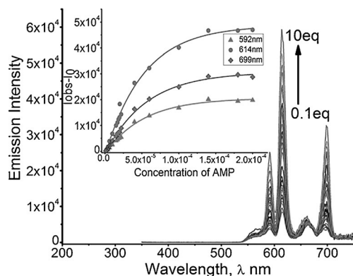
Figure 4. Evolution of the \text{Eu}^{\text{III}} -centered emission upon titration of [\text{Eu}_2(\text{H}_2\text{L})_2(\text{NO}_3)_2(\text{H}_2\text{O})_4](\text{NO}_3)_4 ( 2 \times 10^{-5} \text{ M} ) with AMP in HEPES buffer (10 mM, pH 7.4) at \lambda_{\text{ex}} = 320 \text{ nm} , showing the switching-on of emission. Inset: binding isotherms at 592 nm, 614 nm and 699 nm ( I_{\text{obs}} is the observed emission intensity and I_0 is the initial emission intensity before adding AMP).
